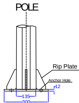
BASE PLATE Side View
