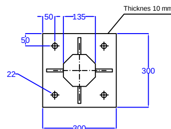
BASE PLATE Top View
